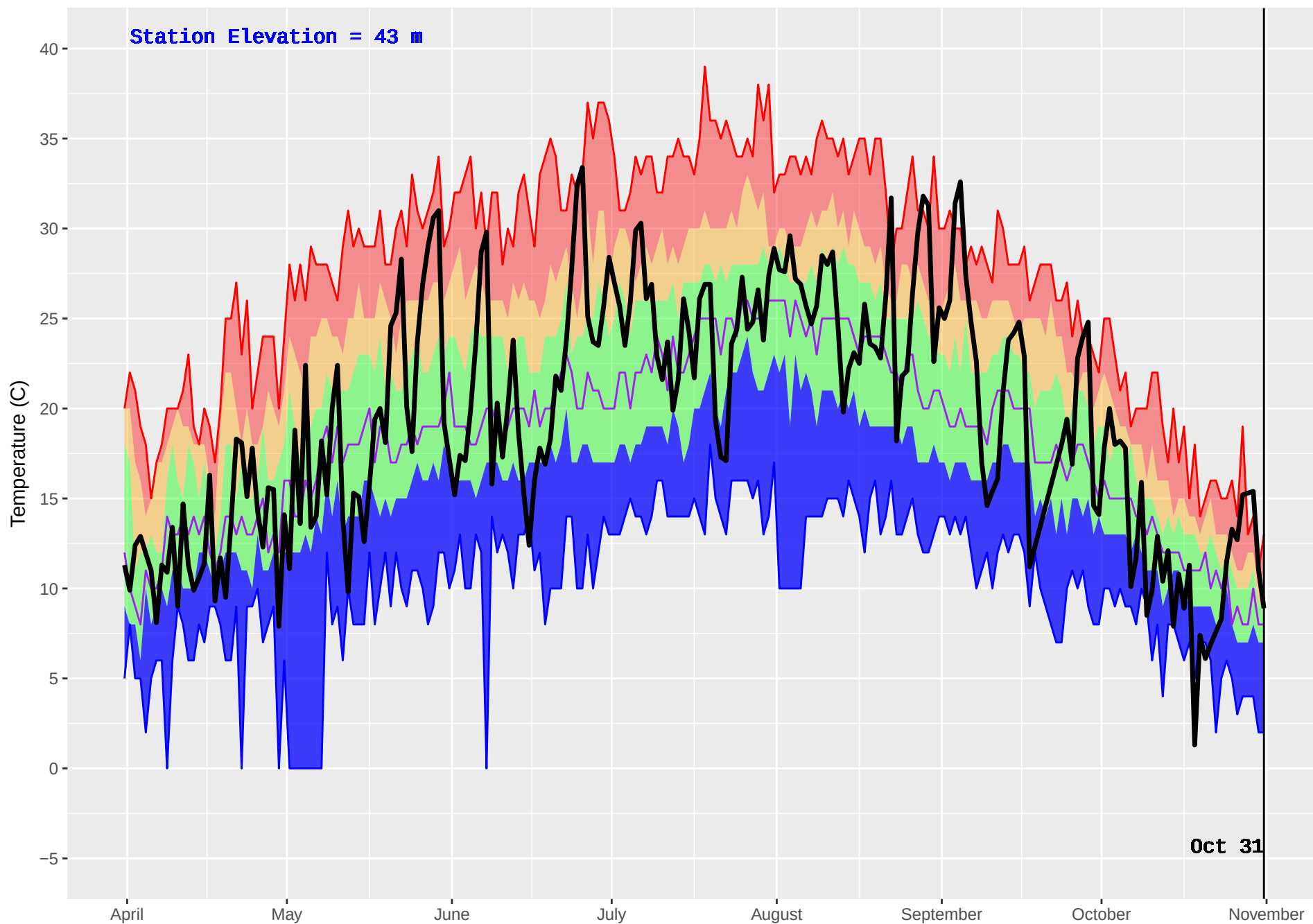
TOBA CAMP (75) : Historical (1970–2016) and Current (2017) Noon Temperature
