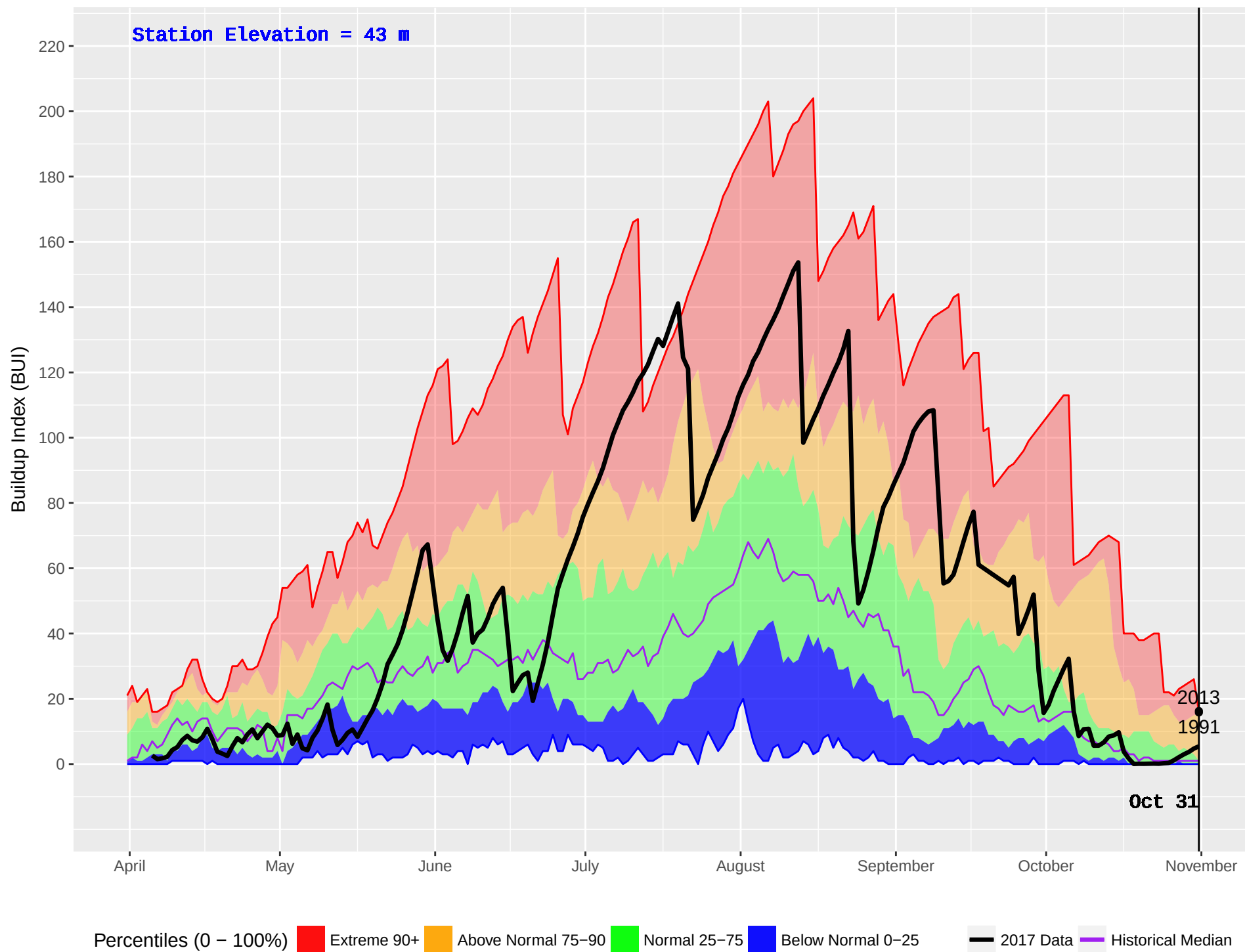
TOBA CAMP (75) : Historical (1970–2016) and Current (2017) Noon Buildup Index (BUI)
